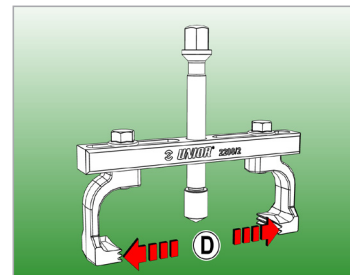
SHORT BEAM, min. D = Ø75mm, max. D = Ø150mm LONG BEAM, min. D = Ø125mm, max. D = Ø240mm
