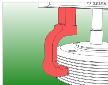
Disassembly of double height driver pulley with ribbed jaws and additional extensions • Demontaža dvojne debeline jermenice z snemalno šapo z ozobjem ter nastavkom
