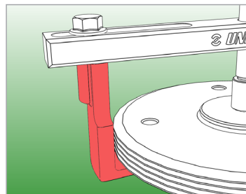
Disassembly of driver pulley with hook jaw • Demontaža jermenice z snemalnim kavljem
