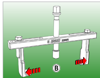
SHORT BEAM, min. B = Ø38mm, max. B = Ø130mm LONG BEAM, min. B = Ø90mm, max. B = Ø205mm
