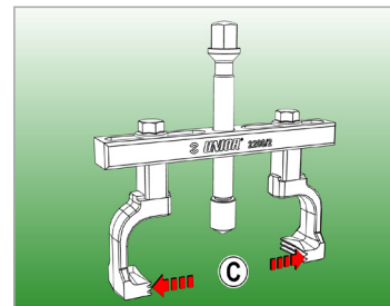
SHORT BEAM, min. C = Ø75mm, max. C = Ø150mm LONG BEAM, min. C = Ø125mm, max. C = Ø240mm
