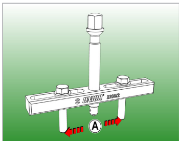
SHORT BEAM, min. A = Ø40mm, max. A = Ø160mm LONG BEAM, min. A = Ø90mm, max. A = Ø240mm
