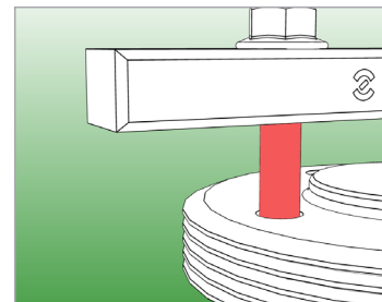
Disassembly of driver pulley with two M10 screws • Demontaža jermenice s pomočjo dveh vijakov M10
