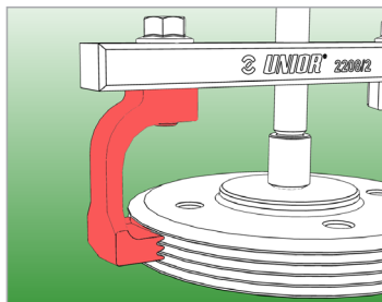
Disassembly of driver pulley with ribbed jaws • Demontaža jermenice z snemalno šapo z ozobjem
